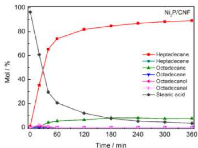
Figure 5. Stearic acid and products concentration (%mol) over time for Ni_2P/CNF for stearic acid deoxygenation (250 mg catalyst, 2 g stearic acid, 50 mL solvent, 30 bar H_2 , T = 350\text{ }^\circ C ).
