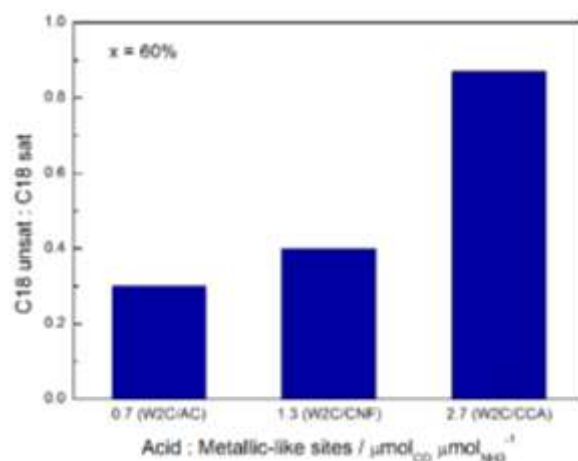
Figure 9. Effect of the acid/metallic site ratio on the C18-unsat:C18-sat ratio at 60% conversion during stearic acid HDO (250 mg catalyst, 2 g stearic acid, 50 mL solvent, 30 bar H 2 , 350 °C).
