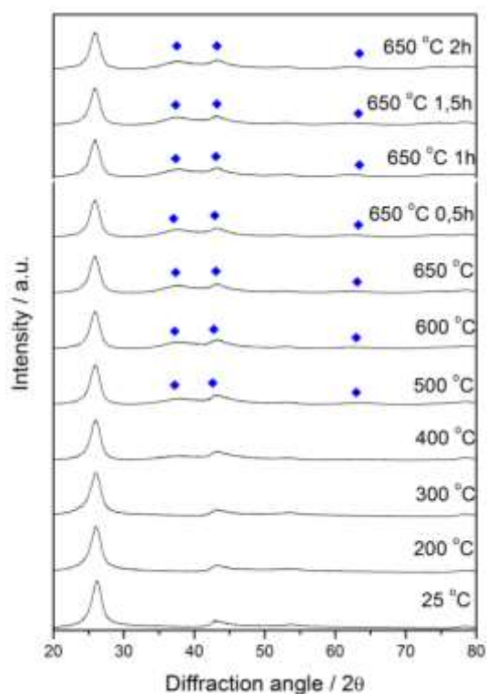
Figure. 2. In-situ XRD diffractogram for 7.5 wt% Mo 2 C/CNF synthesized via carburization with 20% CH 4 /H 2 gas mixture (◆ indicates cubic \alpha -MoC 1-x ).
