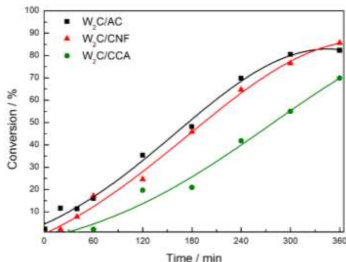
Figure 5. Stearic acid conversion over tungsten carbide supported on AC, CNF and CCA (250 mg catalyst, 2 g stearic acid, 50 mL solvent, 30 bar H 2 , 350 °C).
