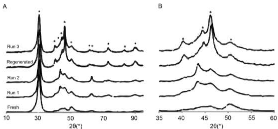
Figure 5. (a) full X-ray diffraction patterns and (b) zoomed in X-ray diffraction patterns of fresh \text{W}_2\text{C}/\text{CNF} (fresh), spent \text{W}_2\text{C}/\text{CNF} (run 1), reused \text{W}_2\text{C}/\text{CNF} (run 2), spent \text{W}_2\text{C}/\text{CNF} after reactivation at 1000 °C (regenerated), and spent reactivated \text{W}_2\text{C}/\text{CNF} (run 3). Reflections are given for graphitic carbon ( \bullet ), \text{XO}_2 ( \blacksquare ), and \text{X}_2\text{C} ( \blacktriangle ), with \text{X} = \text{W} or \text{Mo} [53].
