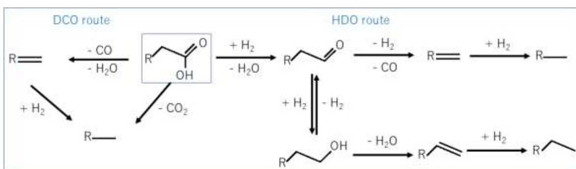
Figure 9. Scheme of possible reaction pathways for stearic acid hydrodeoxygenation over nickel phosphide catalysts, adapted from [35, 36].
