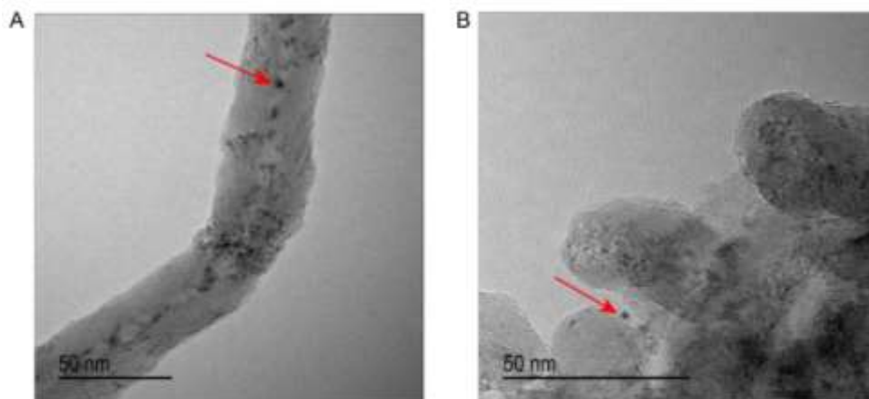
Figure 3. HR-TEM images of A) \alpha - \text{MoC}_{1-x} /CNF and B) \beta - \text{Mo}_2\text{C} /CNF.
