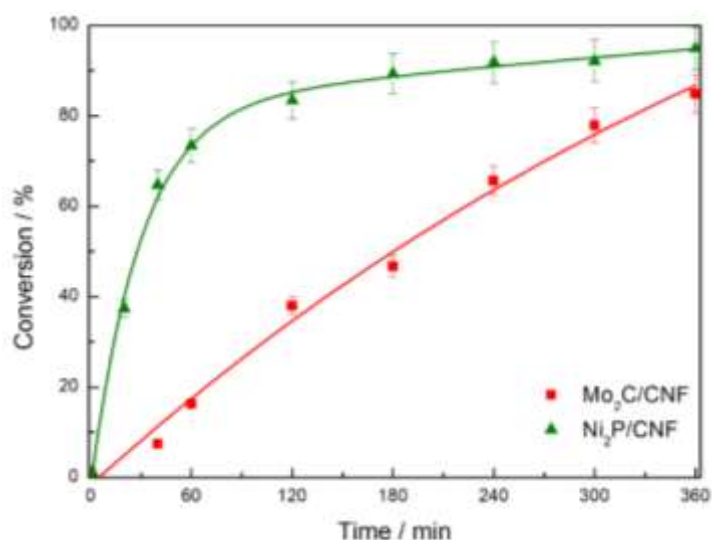
Figure 4. Stearic acid conversion over Mo 2 C/CNF and Ni 2 P/CNF (250 mg catalyst, 2 g stearic acid, 50 mL solvent, 30 bar H 2 , T = 350 °C).
