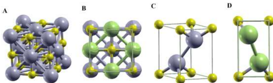
Figure 11. A) Unit cell of fcc structure; B) Atomic configuration for (001) plane of fcc structure; C) Unit cell of hcp structure and D) Atomic configuration for (100) plane of hcp structure. Blue atoms are Mo, yellow atoms are C and green atoms are exposed Mo.
