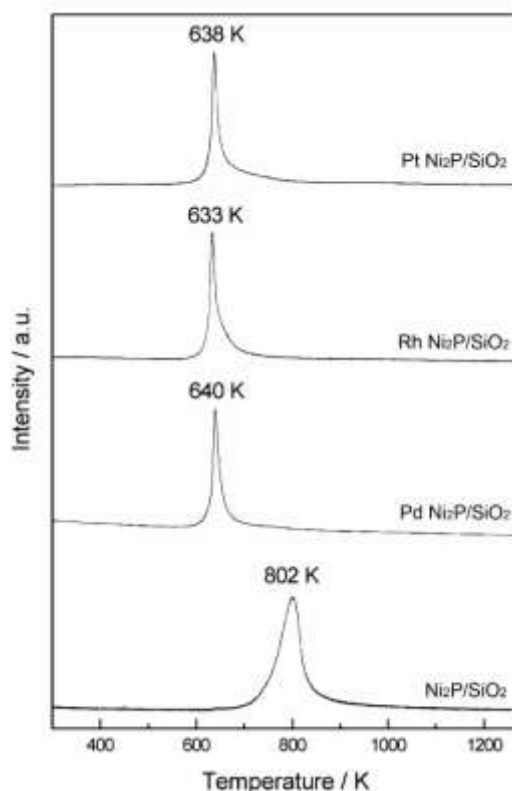
Figure 2. Water formation profiles during TPR of \text{Ni}_2\text{P}/\text{SiO}_2 , Pd \text{Ni}_2\text{P}/\text{SiO}_2 , Rh \text{Ni}_2\text{P}/\text{SiO}_2 and Pt \text{Ni}_2\text{P}/\text{SiO}_2 .
