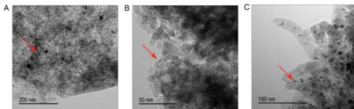
Figure 2. HR-TEM images of A) W_2C/AC , B) W_2C/CCA and C) W_2C/CNF .
