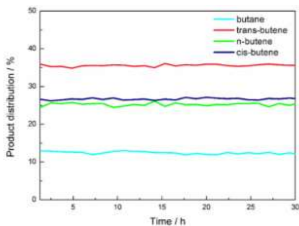
Figure 7. Product distribution for Pd 6 P/SiO 2 in thiophene HDS reaction at 593 K and 1 atm. Butane (light blue), 1-butene (green), trans-2-butene (red) and cis-2-butene (dark blue).
