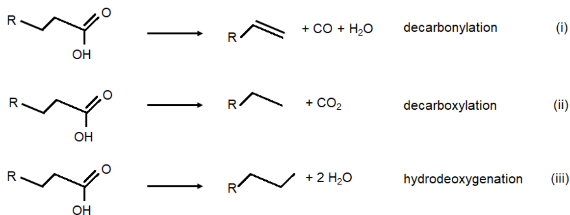
Figure 4. Overview of possible fatty acid deoxygenation reactions [16].
