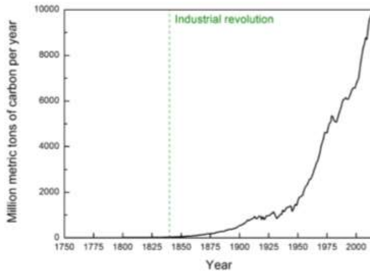
Figure 1. Annual global fossil-fuel carbon emission [Adapted from 1].
