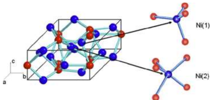
Figure 7. Ni(1) and Ni(2) sites in Ni 2 P [18].
