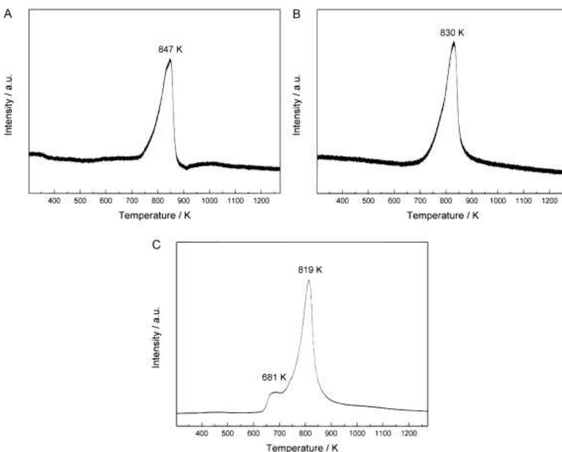
Figure 3. – Water formation profiles during TPR of the samples in A) 1 o configuration, B) 2 o configuration and C) 3 o configuration.
