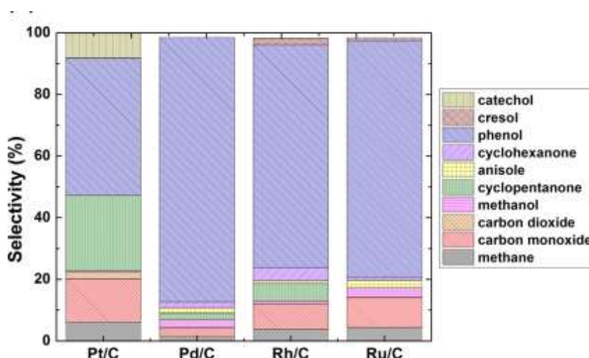
Figure 1. Distribution of major products in deoxygenation of guaiacol using carbon supported noble metal catalysts (Reprinted with permission from [34]. Copyright 2018 American Chemical Society).
