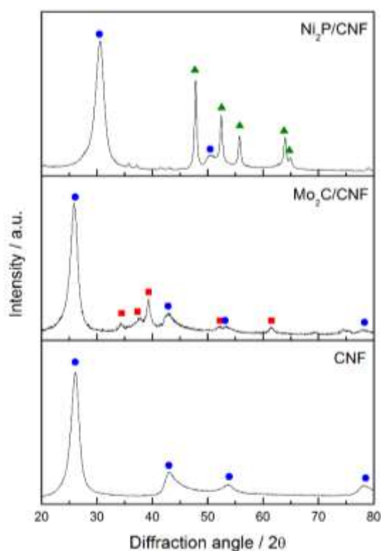
Figure 1. XRD diffractogram for ● CNF (using copper radiation), ■ \text{Mo}_2\text{C}/\text{CNF} (using copper radiation) and ▲ \text{Ni}_2\text{P}/\text{CNF} (using cobalt radiation). Due to the use of different sources the peaks appear at different positions for the same phase (most clearly seen for CNF).
