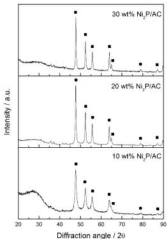
Figure 1. X-ray diffractograms of 10, 20 and 30 wt% Ni 2 P/AC.
