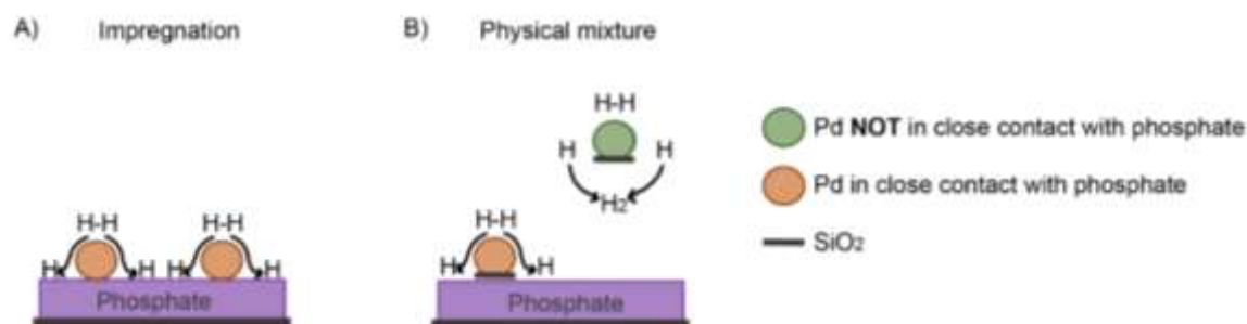
Scheme 3. Hydrogen spillover phenomena when a) PdO is impregnated on \text{Ni}_x\text{P}_y\text{O}_z/\text{SiO}_2 and b) PdO and \text{Ni}_x\text{P}_y\text{O}_z/\text{SiO}_2 are physically mixed.
